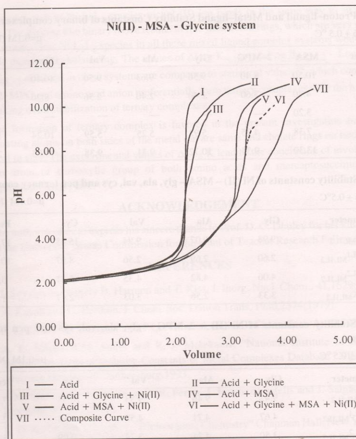
Fig 1. Potentiometric titration curves of Ni (II)-MSA-Glycine system
